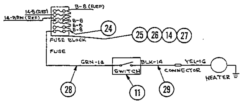
WIRING DIAGRAM
